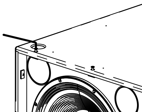
Figure 7.6: Bolt replacement
