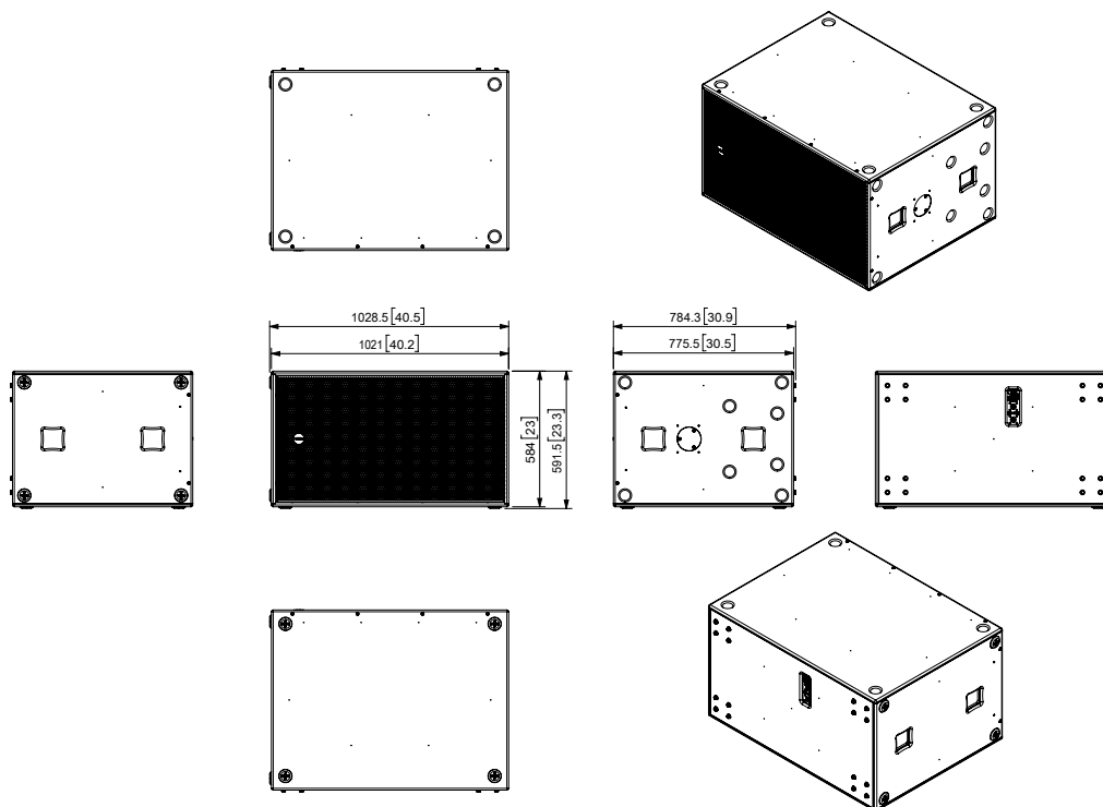
Figure 4.1: Dimensions
