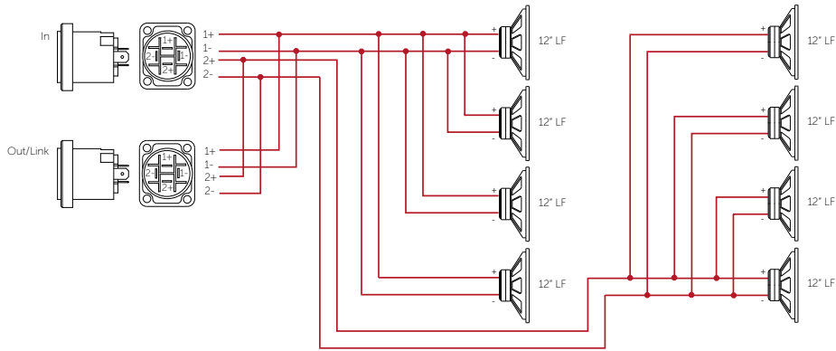
Figure 5.1: Wiring diagram
