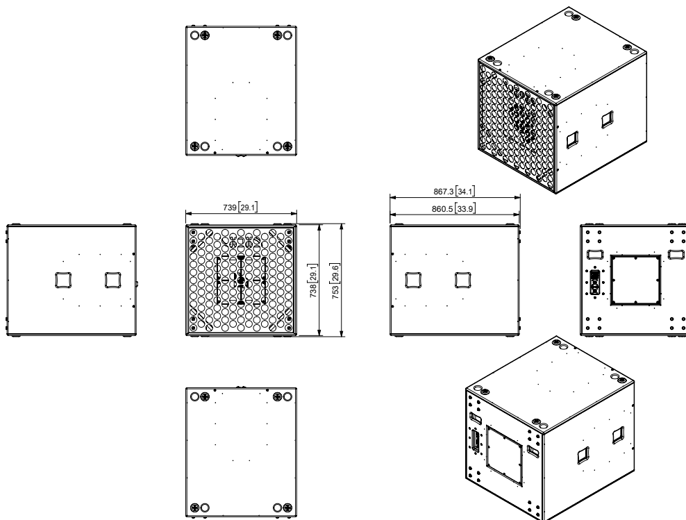
Figure 4.1: Dimensions
