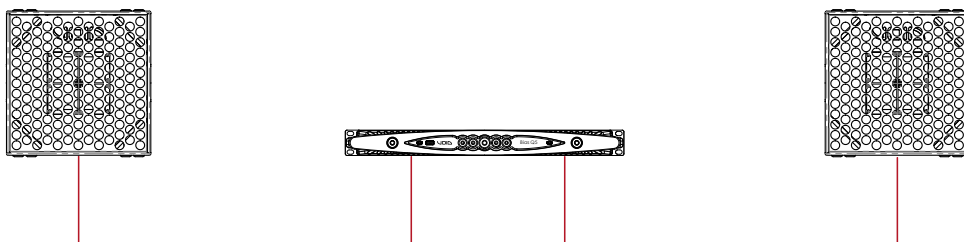
Figure 5.3: 2 x Nexus X: 4 Ω per channel / 1 amplifier
