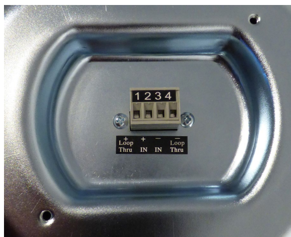
Figure 7.5: Terminal layout
