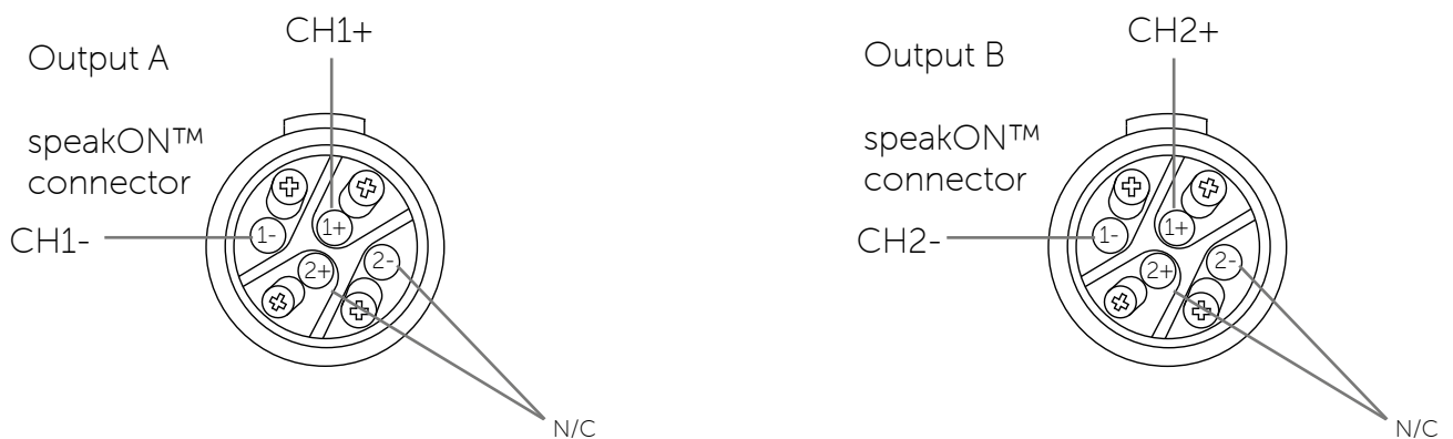
Figure 4.12: Channel 1 and 2 speakON™ connector diagram. Note: pins 2+/2- are not connected.
