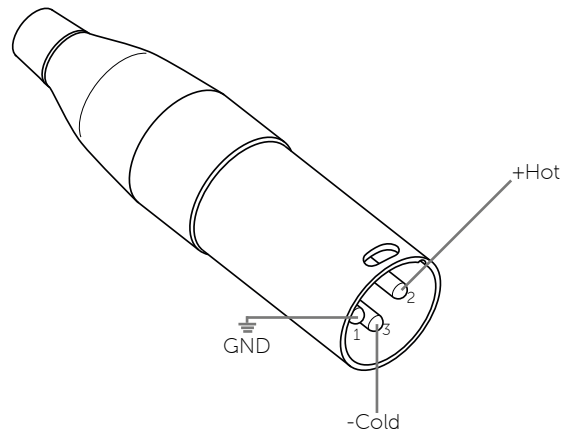
Figure 4.10: XLR-M diagram
