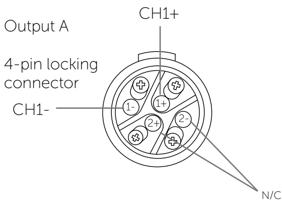
Figure 4.8: Channel 1 and 2 4-pin locking connector diagram. Note: pins 2+/2- are not connected.
