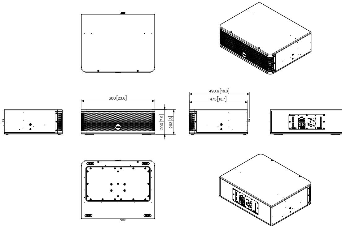
Figure 8.1: Dimensions
