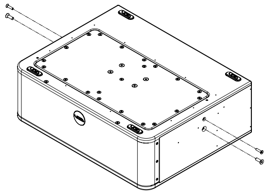
Figure 6.2: Bolt removal
