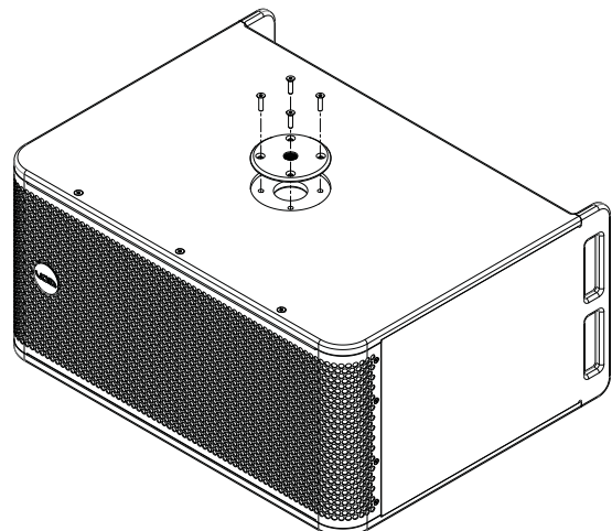
Figure 6.14: Top hat placement
