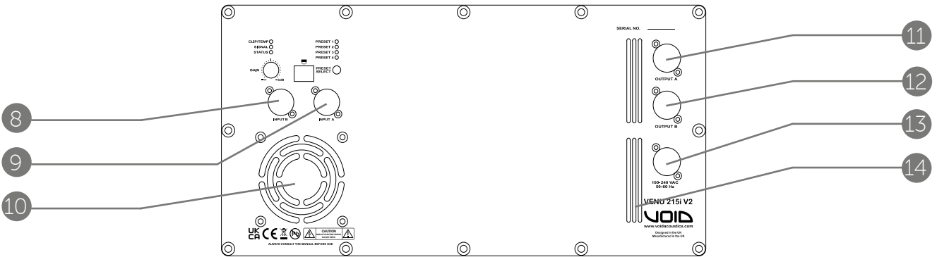
Figure 5.6: Rear panel
