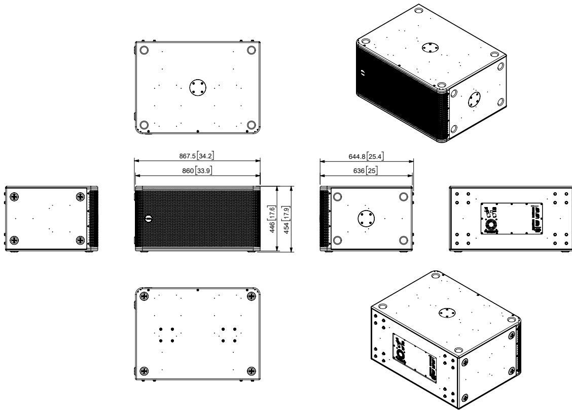
Figure 8.3 Dimensions
