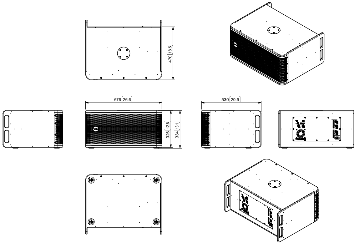
Figure 8.2: Dimensions
