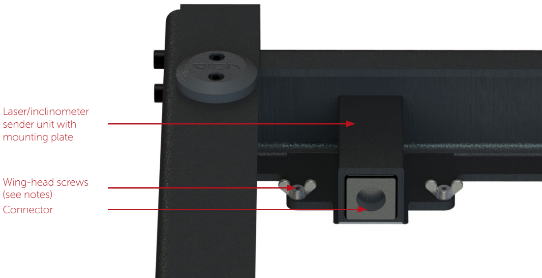
Figure 6.3: Void Arcline 8 Fly Frame laser/inclinometer sender unit mounting
