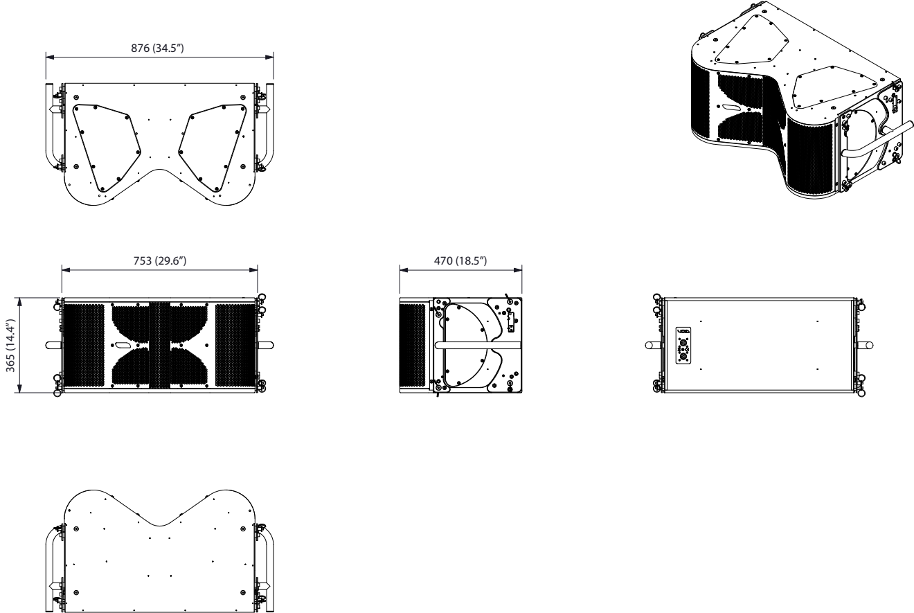
Figure 3.2: Arcline 212 dimensions
