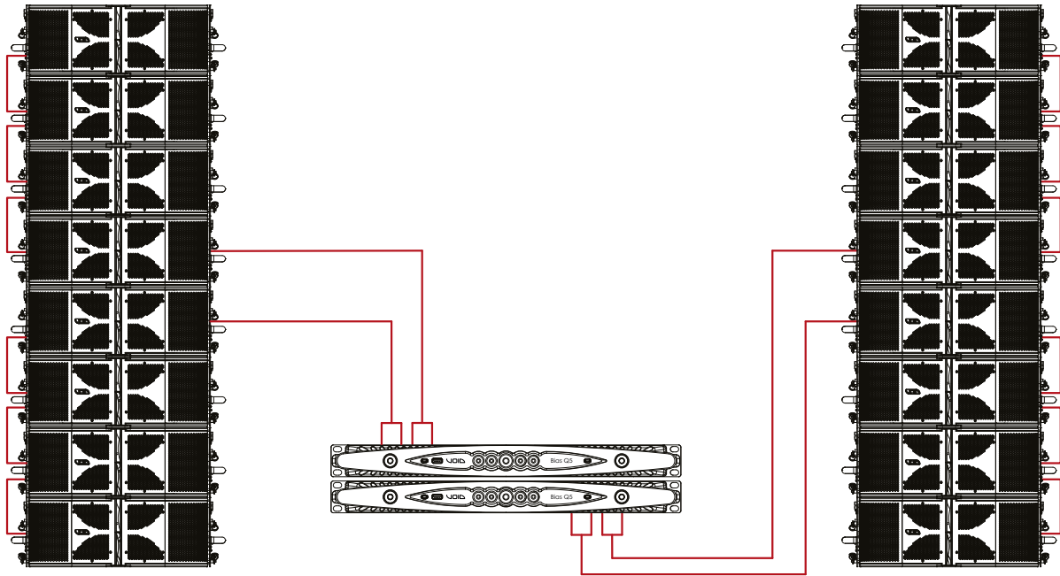
Figure 7.2: 16 Arcline 8
