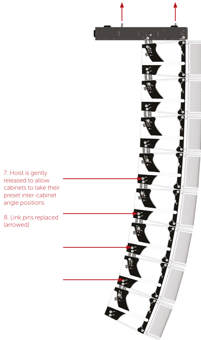
Figure 6.12: Steps 7 – 10 have been completed and the chain hoist and bridle have been removed
