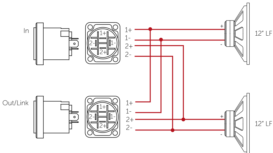
Figure 4.2: Arcline 212 wiring diagram
