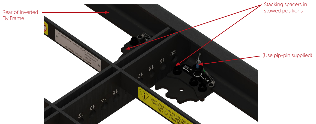
Figure 6.17: Stacking spacers in stowed position for transportation
