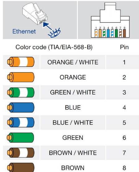
1000BASE-T (4-pair) S/UTP* ethernet cable pinouts suitable for data + AES3 (AESOP) applications. (*Note S/UTP – not U/UTP)
