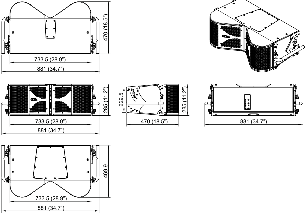
Figure 3.1: Arcline 8 dimensions
