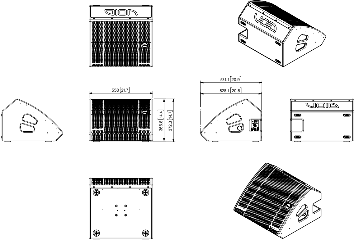
Figure 3.3: Dimensions
