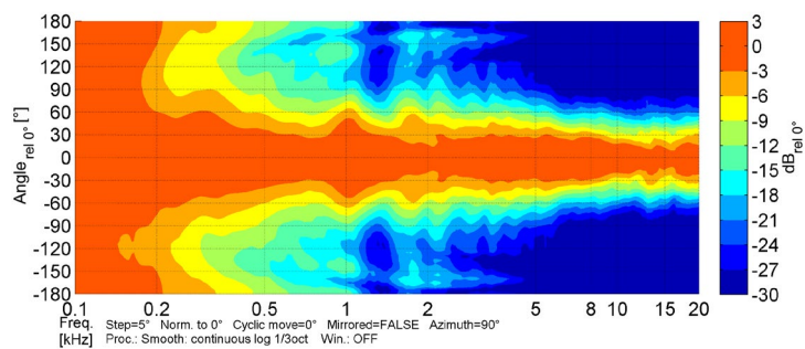
Figure 3.2: Vertical directivity isobars
