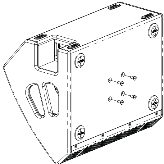
Figure 5.5: Bolt removal
