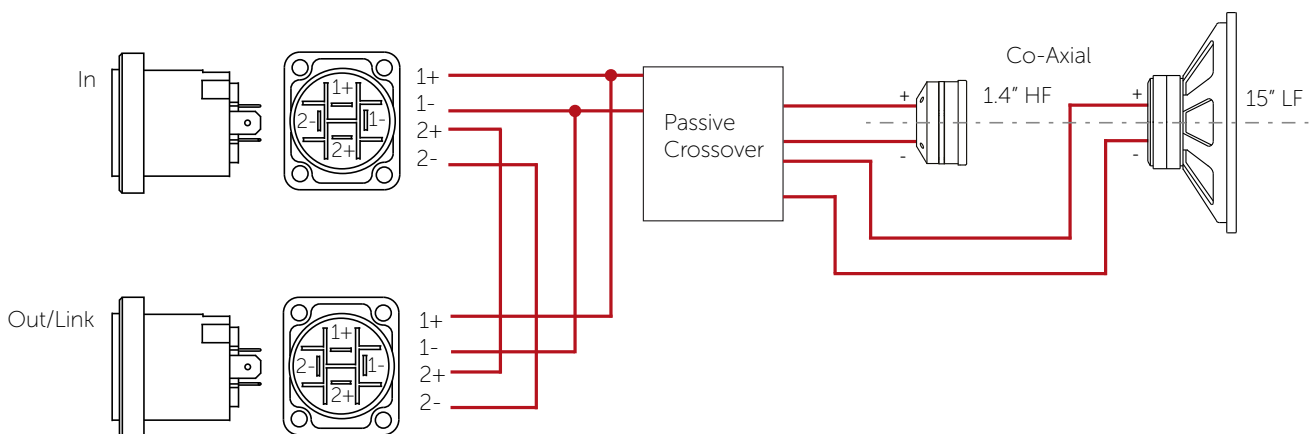
Figure 4.1: ArcM 15 passive mode wiring diagram
