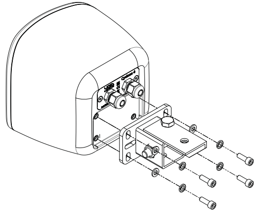
Figure 5.10: Mounting plate
