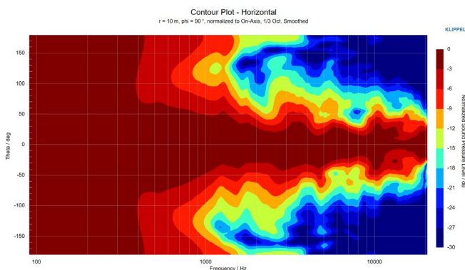
Figure 3.1: Horizontal directivity isobars
