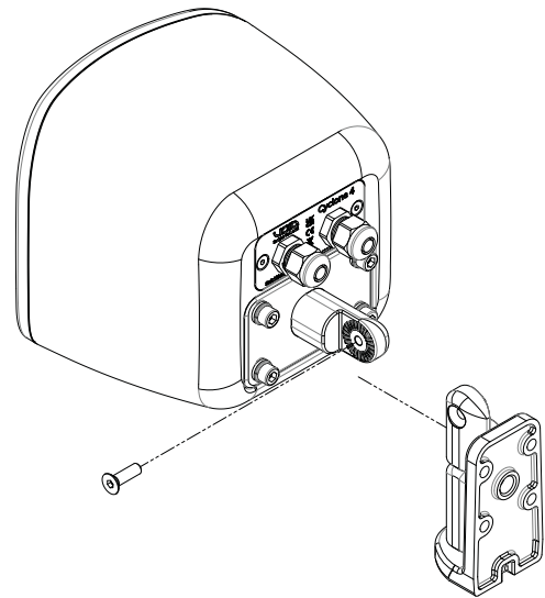
Figure 5.5: Wall mounting
