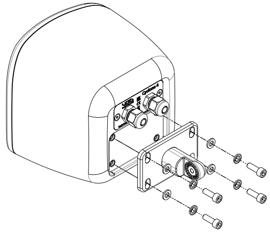
Figure 5.4: Attach plate
