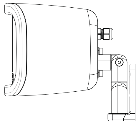
Figure 5.6a: Bracket adjustment
