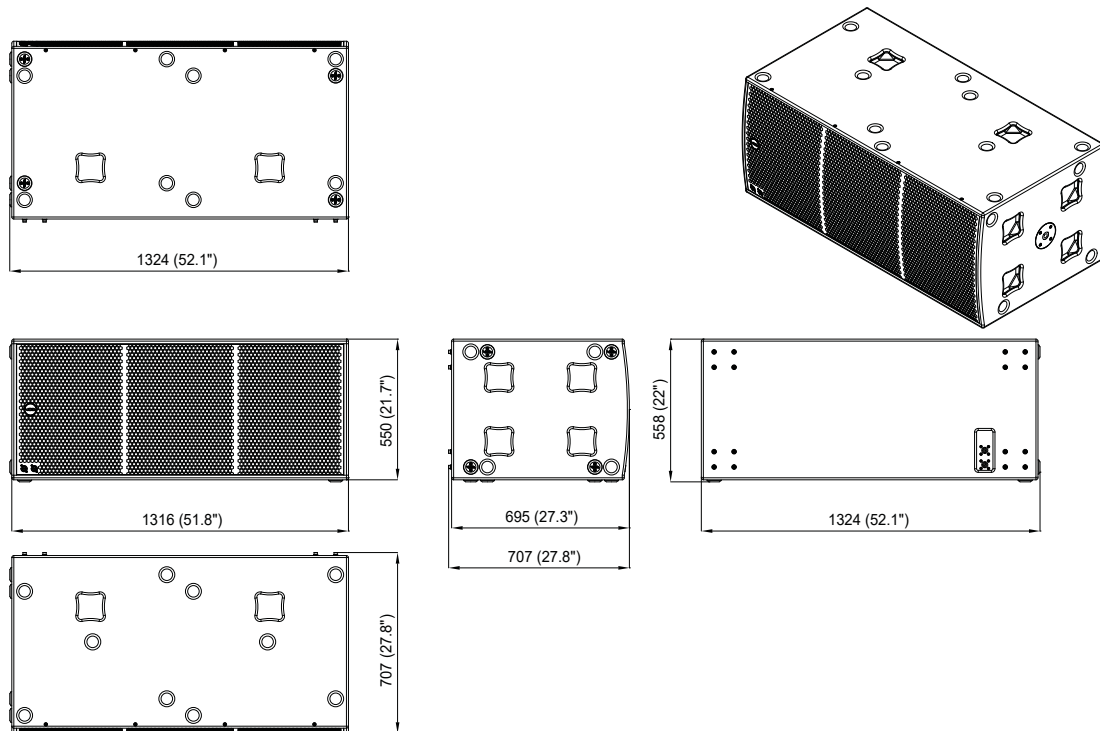
Figure 3.1: Dimensions
