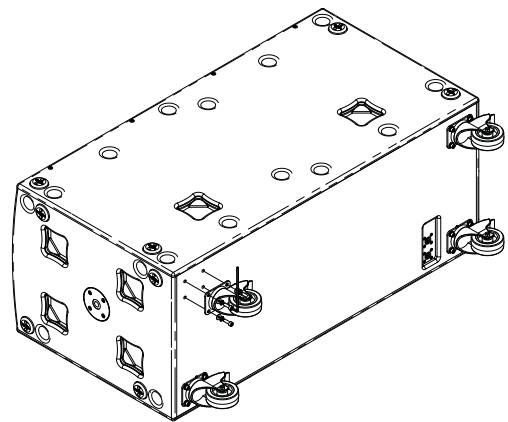
Figure 5.2: Wheel removal
