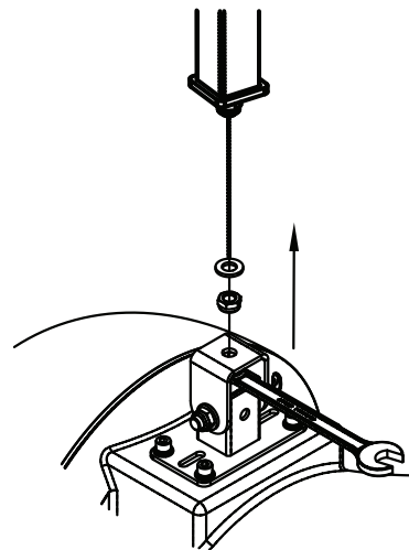
Figure 5.29: Air Vantage truss mount detail
