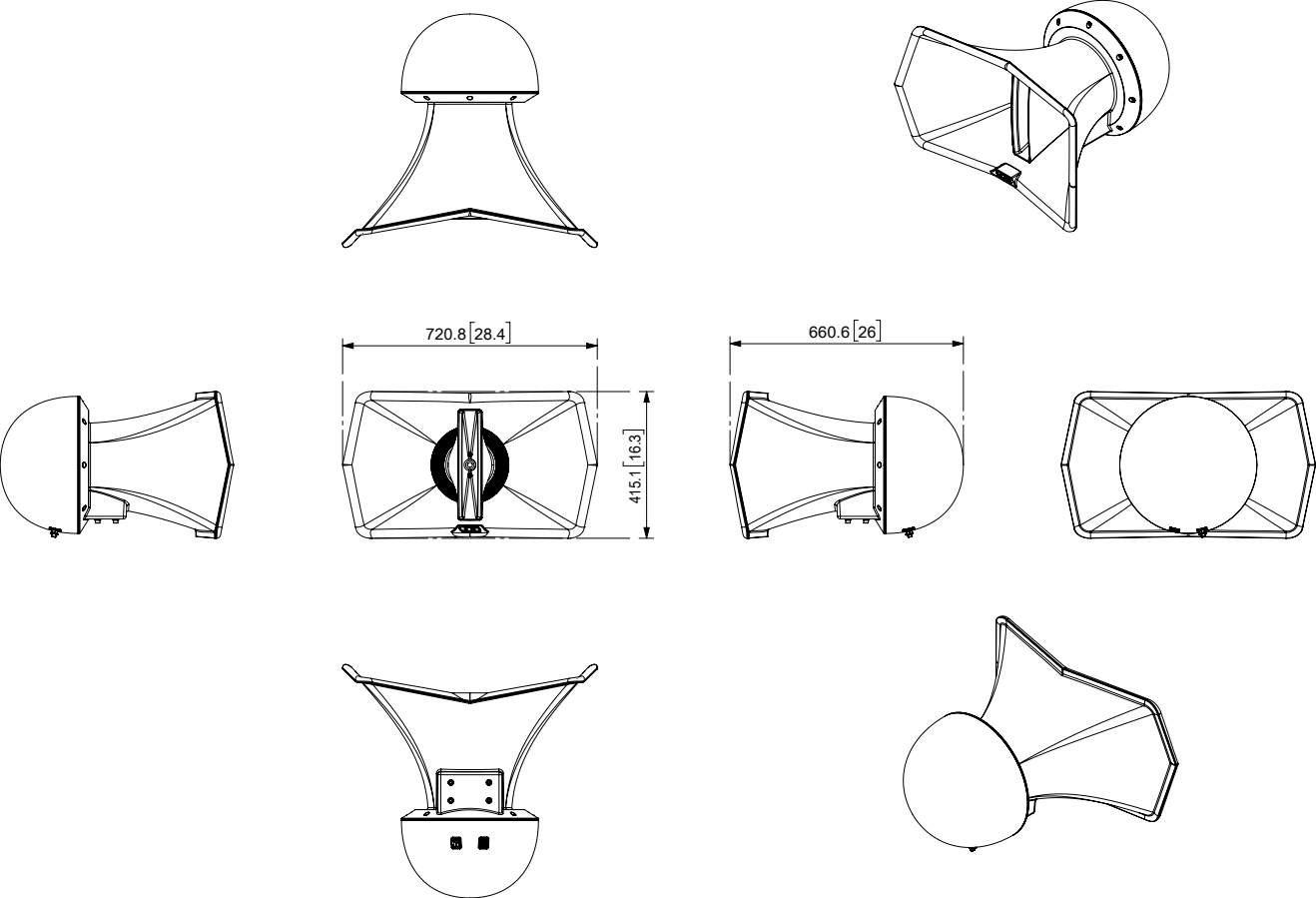
Figure 3.3: Dimensions
