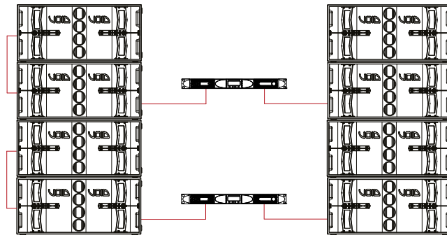
Figure 4.7: 8 x Xair: 2 \Omega per channel/2 amplifier
