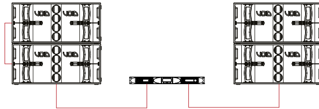
Figure 4.5: 4 x Xair: 2 \Omega per channel/1 amplifier
