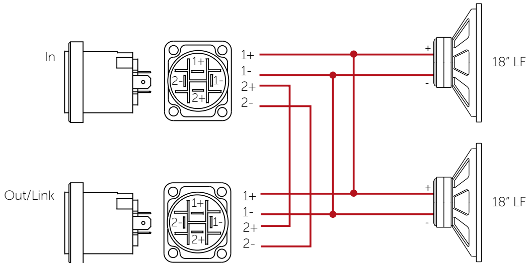
Figure 4.2: Xair wiring diagram
