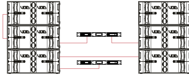
Figure 4.6: 6 x Xair: 2 \Omega per channel/2 amplifier
