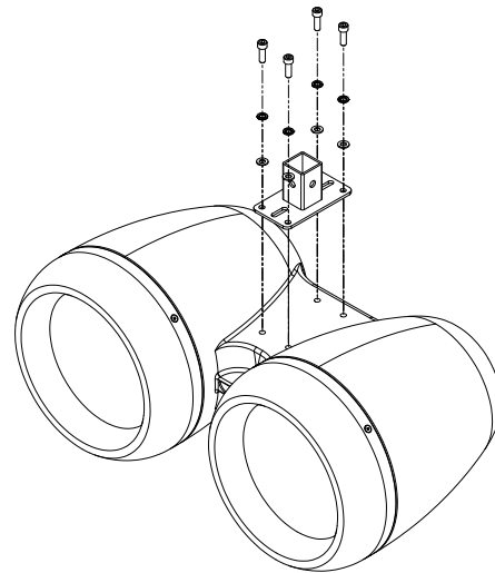
Figure 5.18: T75 attachment
