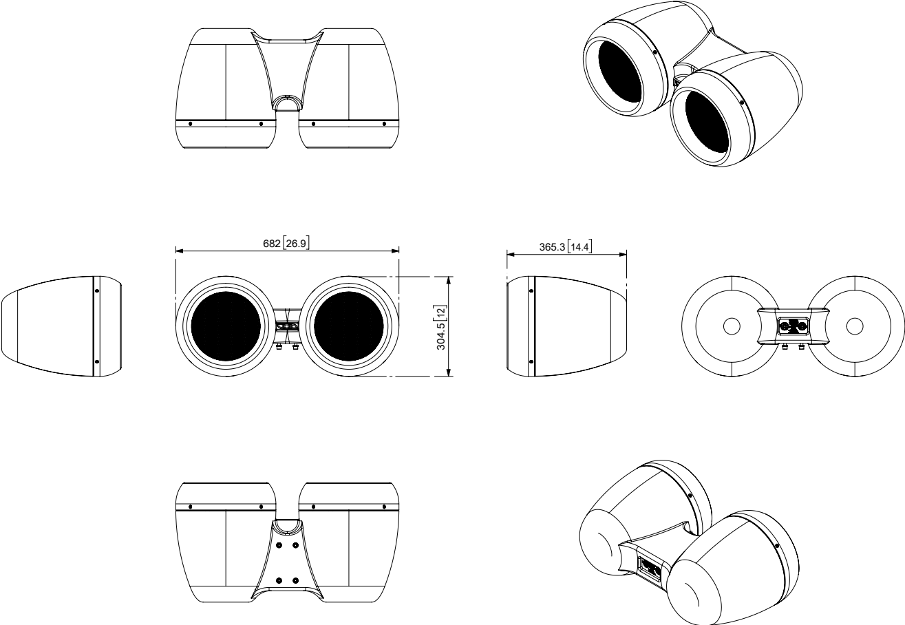
Figure 3.3: Dimensions
