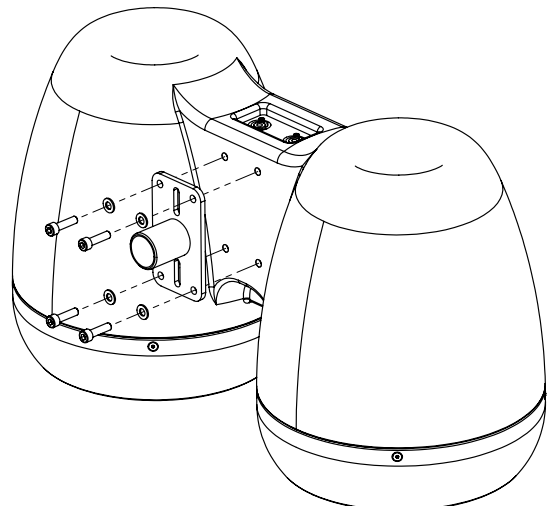
Figure 5.3: T75 pole bracket positioning
